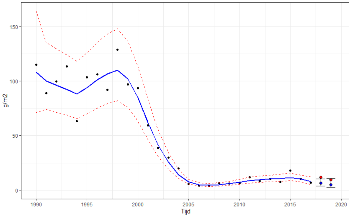
Trend estimate with 95% confidence limits & 95% CI forecast
