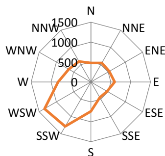
Windrichtingsverdeling station Cabauw
