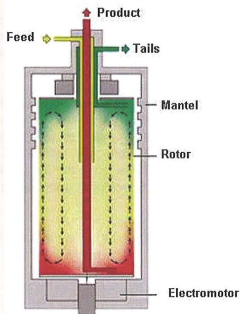
Fig. 1: Ultracentrifuge
