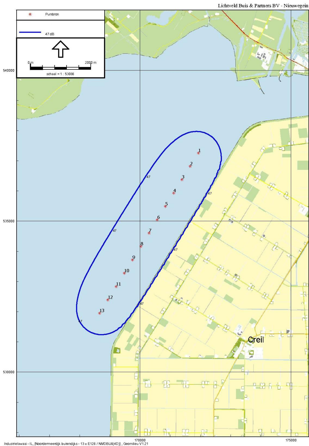
Figuur 5.2 Lden 47 dB contour NMDbu5-8(4D)
