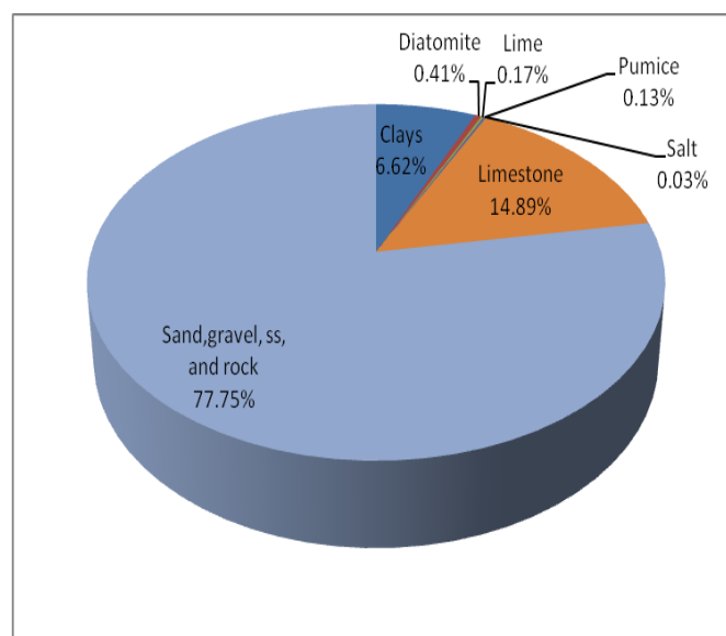
Figure B-5: Costa Rica Minerals Production (Anderson, 2008)
