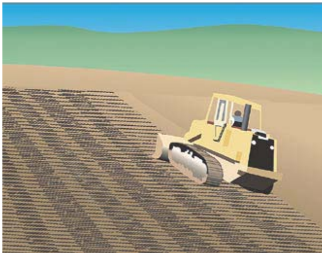
Tread-track slopes up and down hill to improve stability.
