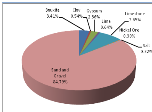
Figure B-7: Dominican Republic – 2005 Non-metallic Mineral Production (Bermúdez-Lugo, 2008 )
