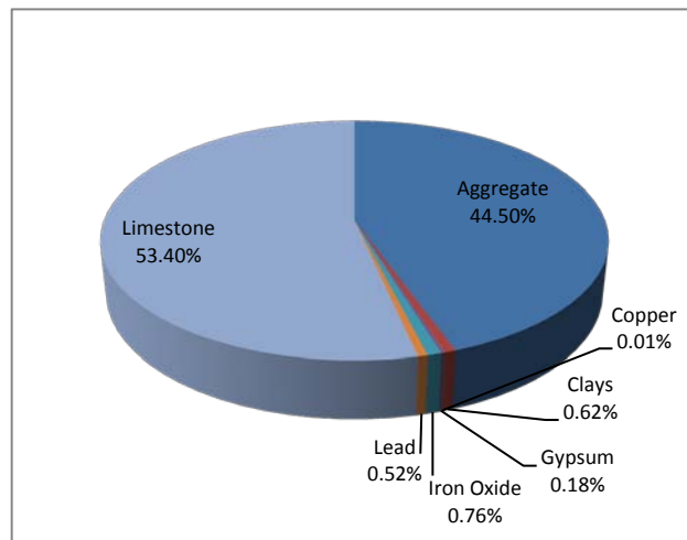
Figure B-10: Honduras - 2006 Non-metallic Mineral Production (Anderson, 2008)
